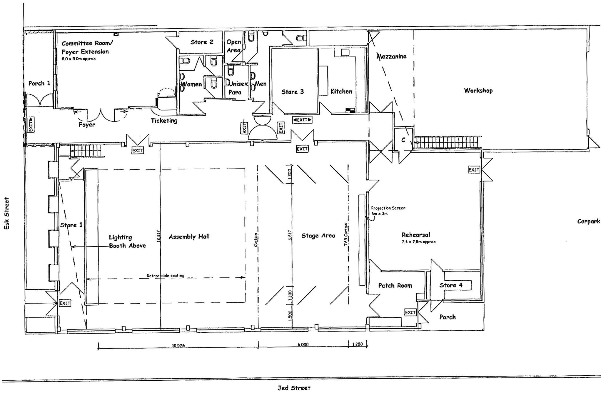
Revised Floor Plan Scale 1:100
